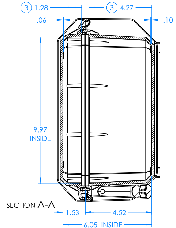
530ML Optional latches with plastic lock
